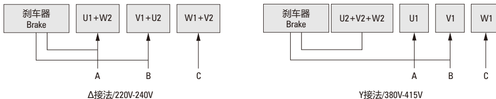
Δ接法/220V-240V
