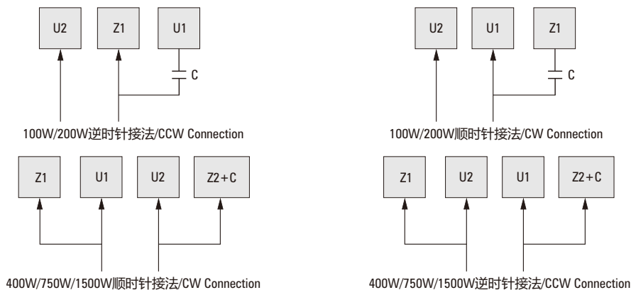
400W/750W/1500W顺时针接法/CW Connection
